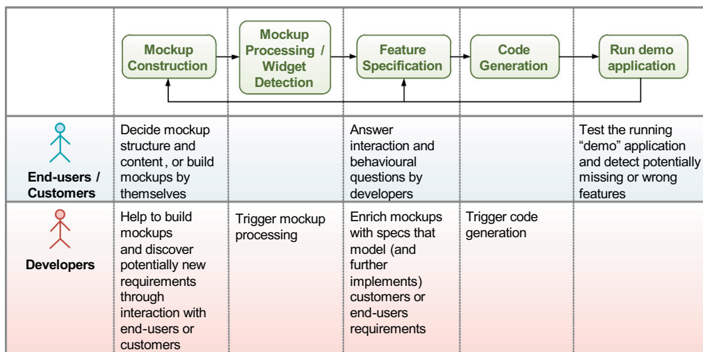
Fig. 3. Actors involved in every MockupDD process stage.
