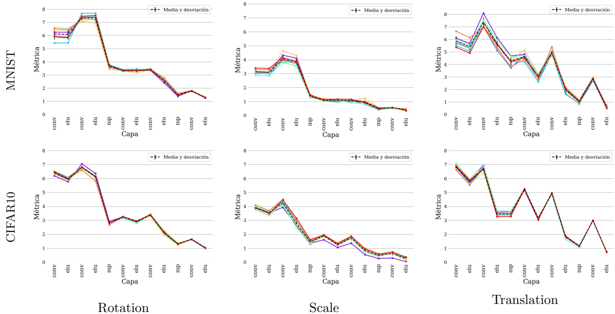
Figure 19: Stability of the Same-Equivariance measure for the SimpleConv model. Each line in each plot corresponds to the invariance obtained by different models with the same architecture. The dashed line shows the mean values. Vertical bars indicate standard deviation.
