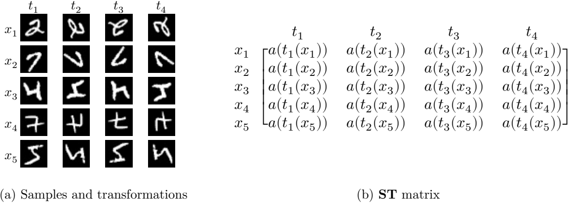
Figure 3: (a) Matrix of samples and their corresponding transformations, for n = 5 samples and m = 4 transformations. (b) Corresponding ST matrix containing the activation values corresponding to each input for a single activation a .
