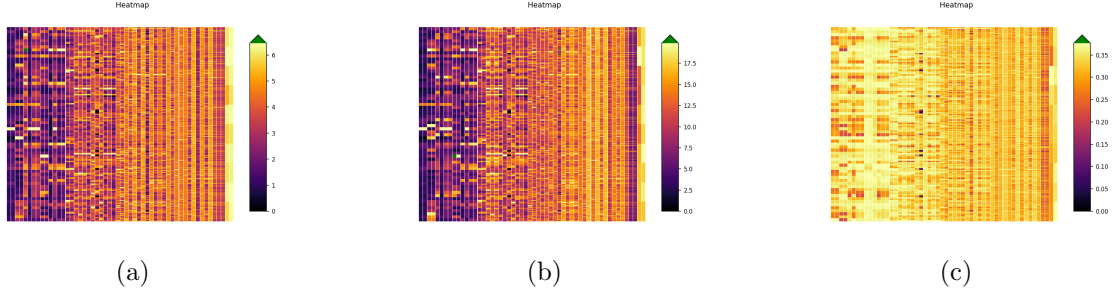
Figure 8: (a) Transformation Variance, (b) Sample Variance and (c) Normalized Variance of each activation of the ResNet model. The transformation set for this example is a set of 16 rotations distributed uniformly between 0^\circ and 360^\circ , and the dataset is the test set of CIFAR10.
