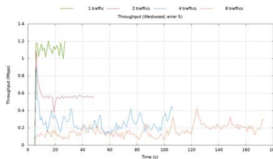
Fig. 24 Throughput vs. Time – 5 errors
