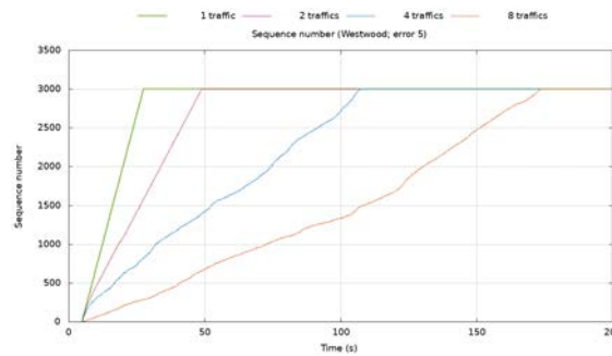
Fig. 25 Sequence N° vs. Time – 5 errors
