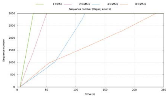
Fig. 35 Sequence N° vs. Time – 5 errors
