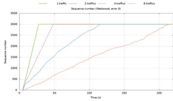
Fig. 23 Sequence N° vs. Time – no errors
