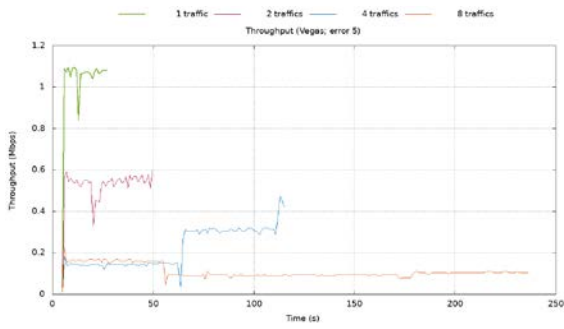
Fig. 34 Throughput vs. Time – 5 errors
