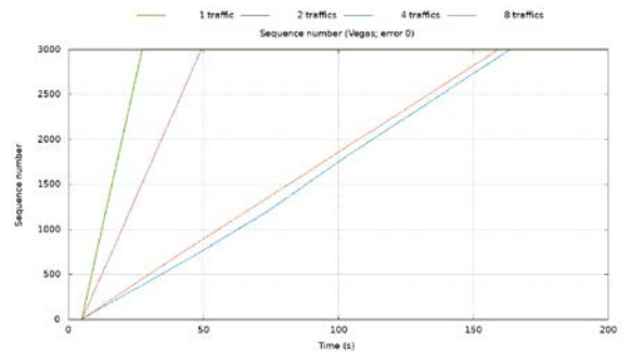
Fig. 33 Sequence N° vs. Time – without errors
