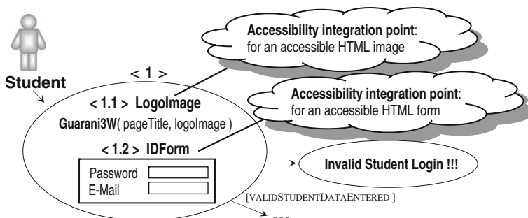
Figure 6 UID with accessibility integration points: login a student given the student's ID and password.
