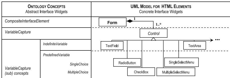
Figure 8 Mapping between some ontology concepts and HTML elements.
