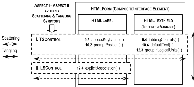
(b) WCAG 1.0 checkpoints crosscutting an HTML form element (Concrete Interface Widget) corresponding to a CompositeInterfaceElement (Abstract Interface Widget)
