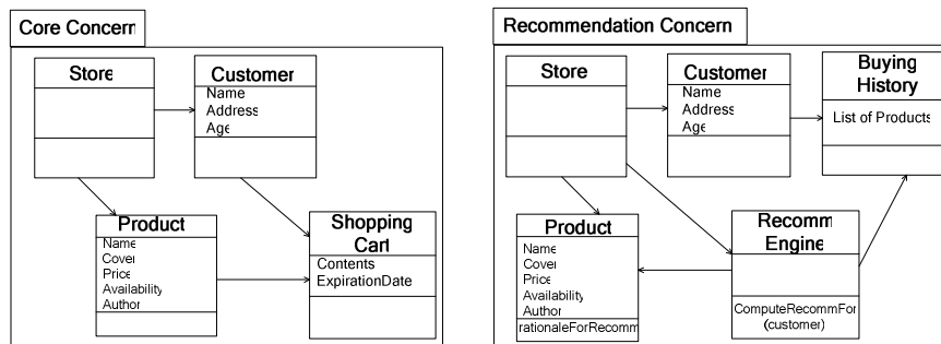
Figure 5: Conceptual Model for the e-store site.
