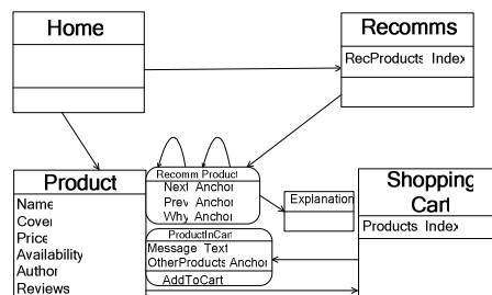
Figure 7: A concern-sensitive navigational schema.
