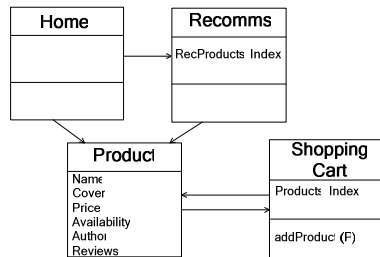
Figure 6: Navigational Schema for the e-store site.
