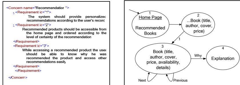
Figure 4: Requirements corresponding to the Recommendation concern.
