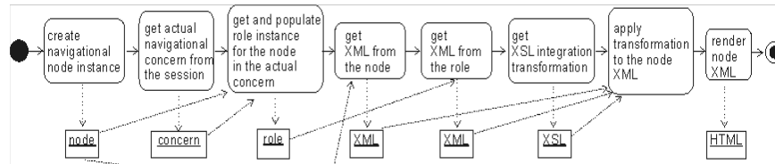
Figure 11: Activity diagram for weaving a role into the core concern.
